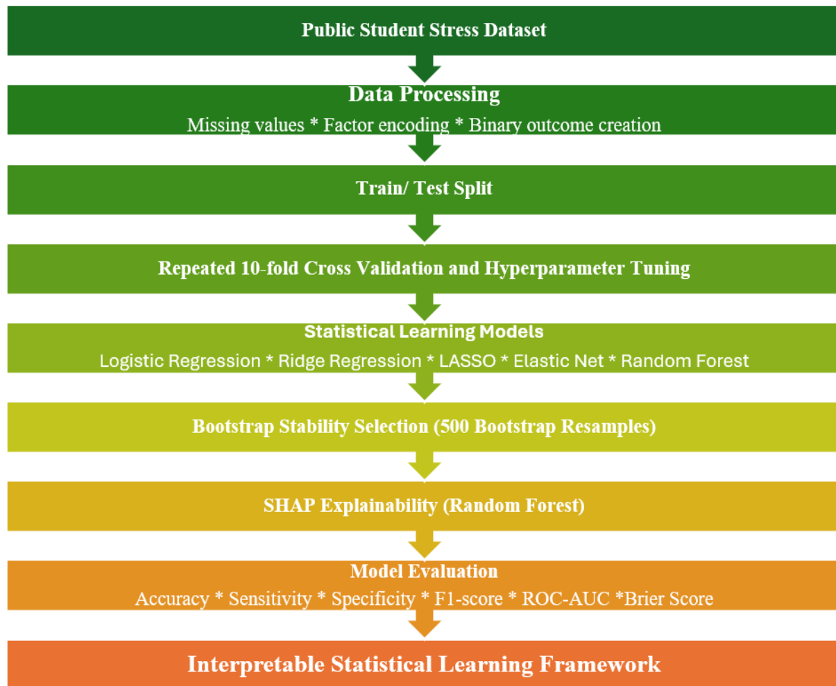
Fig. 1 Workflow of the proposed statistical learning framework.
